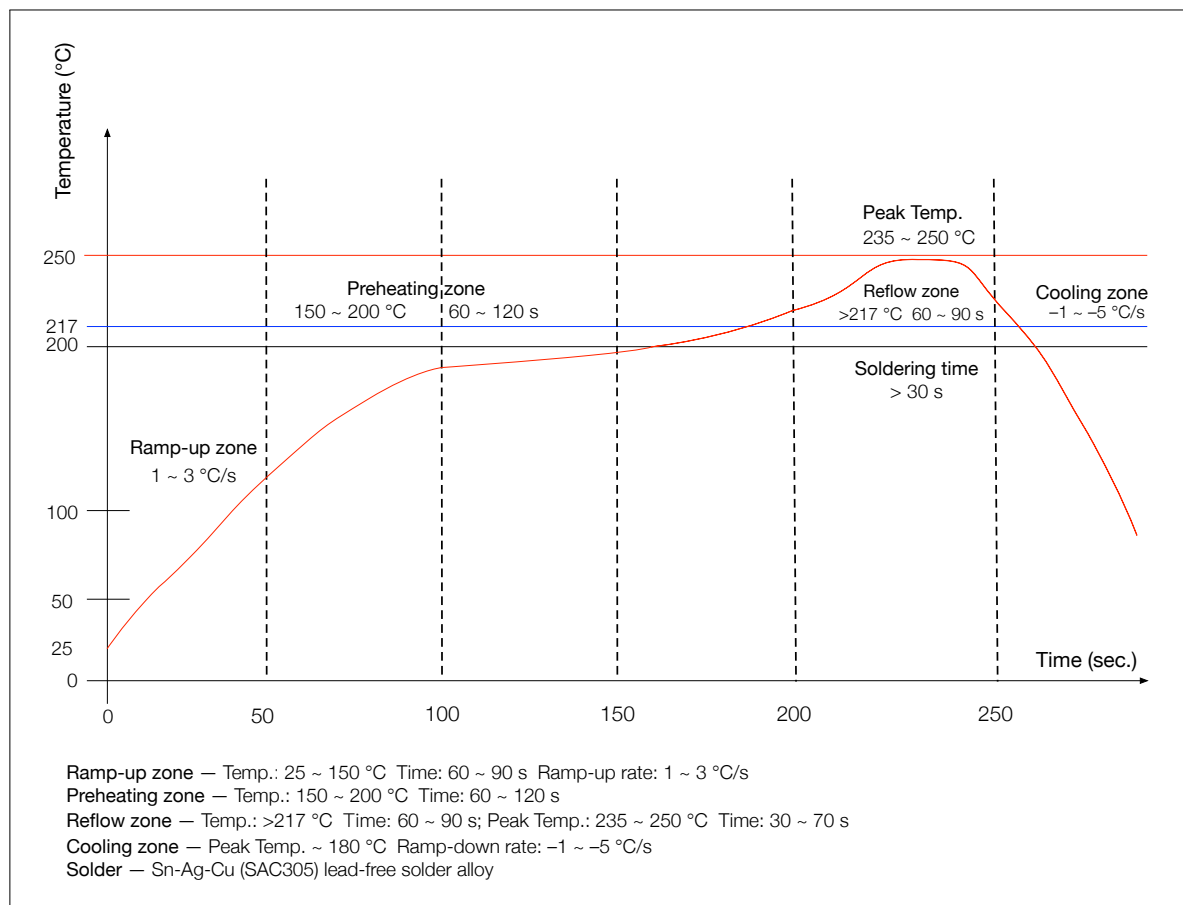
Figure 9: Reflow Profile
