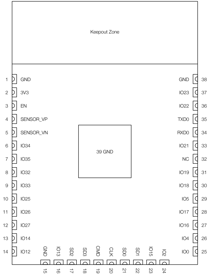
Figure 1: ESP32-WROOM-32 Pin Layout (Top View)
