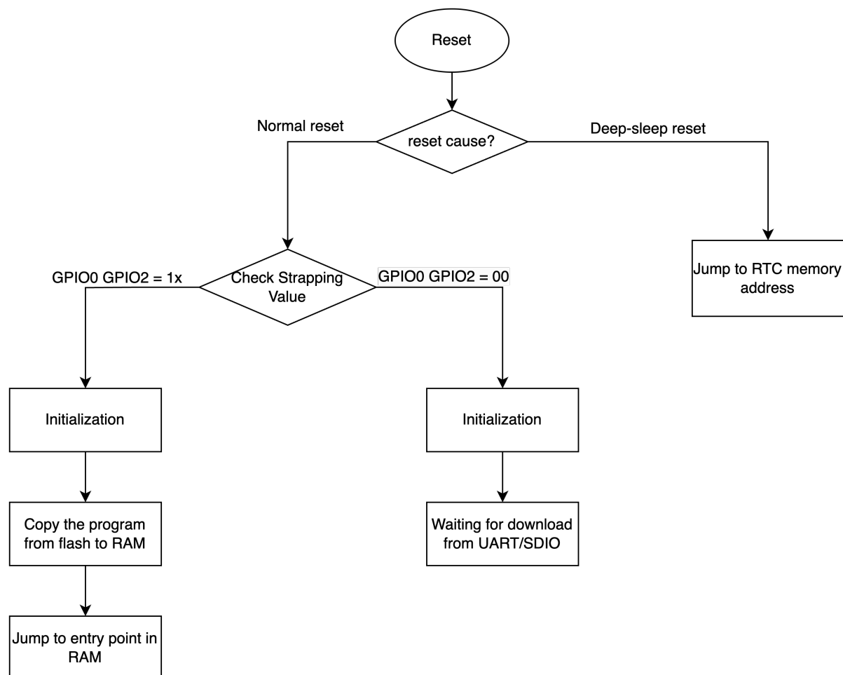
Figure 3: Chip Boot Flow
