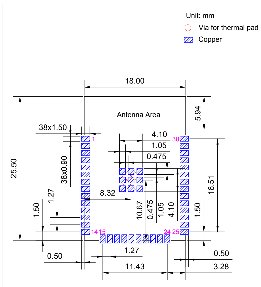
Figure 8: Recommended PCB Land Pattern
