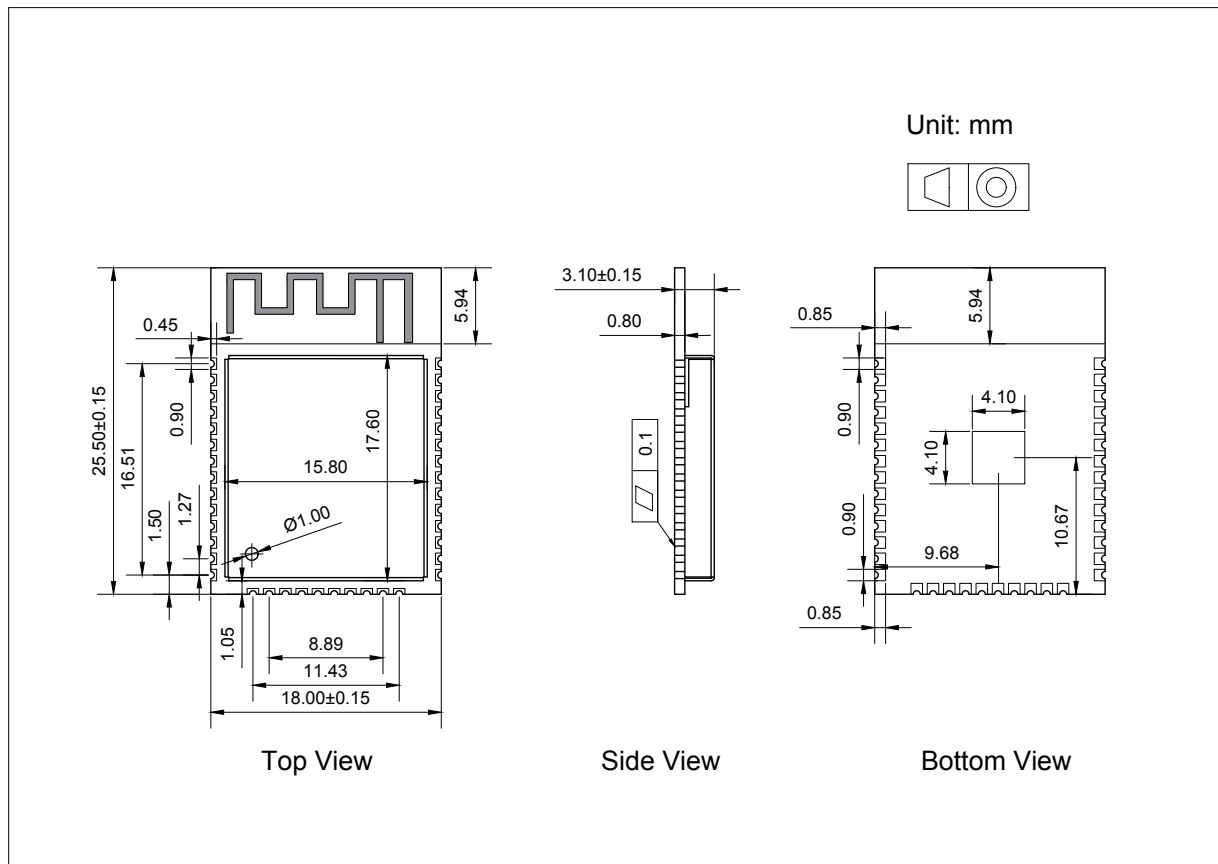
Figure 7: Physical Dimensions
